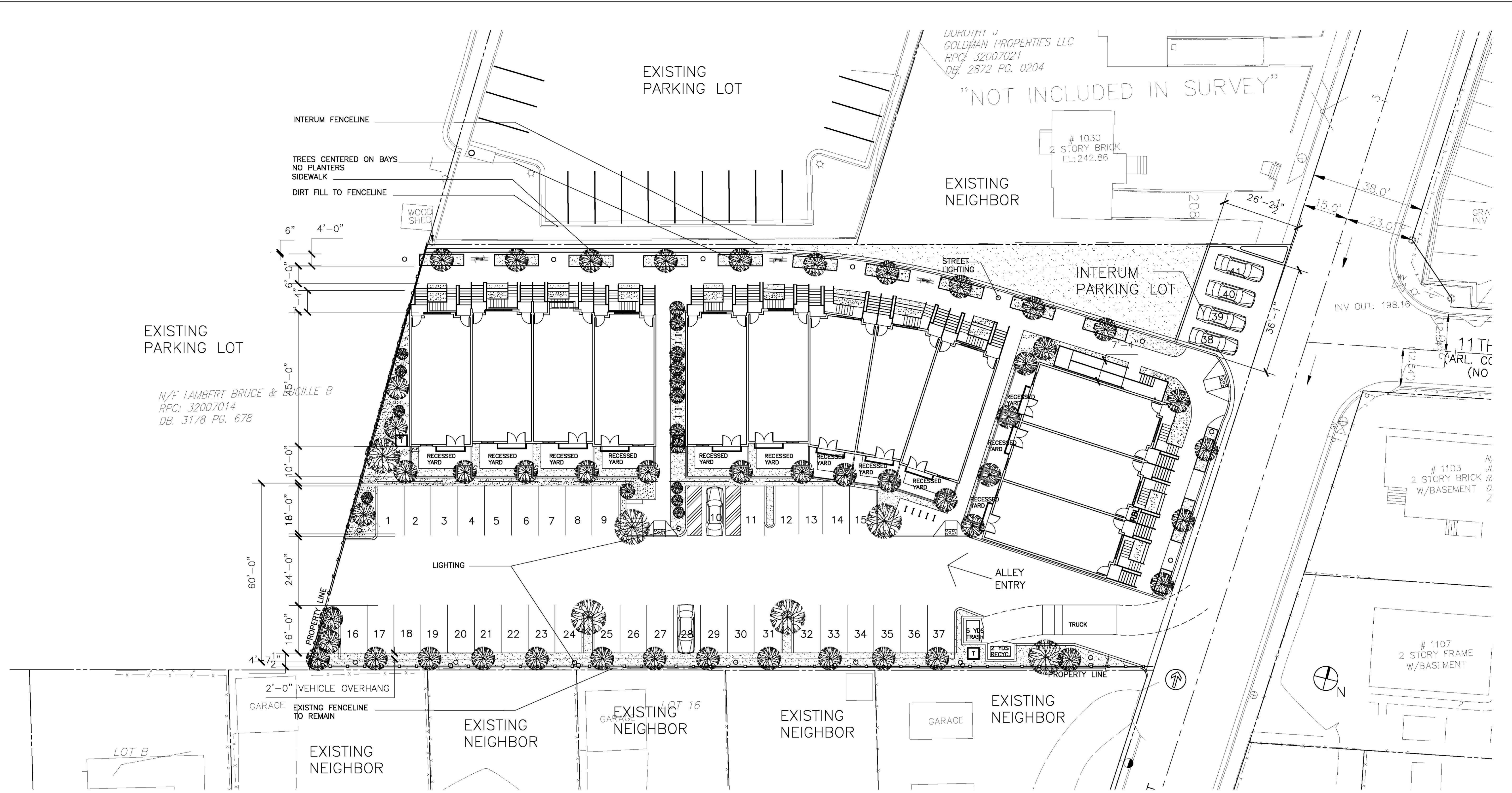
1 INTERIM SITE PLAN Scale 1/16" = 1'-0"
